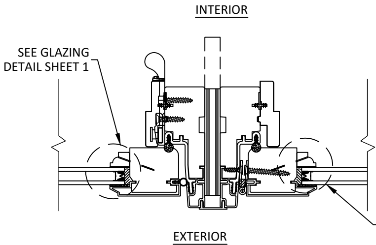
A 9 HORIZONTAL SECTION INSULATED GLASS 1/2" X 3-1/2" MULLION OR 1/2" x 5 3/16"
