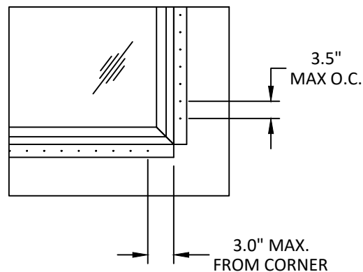
VINYL FIN ANCHORING SINGLE UNIT
