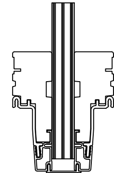
3/4" X 5 3/16" LVL MULL PROFILE
